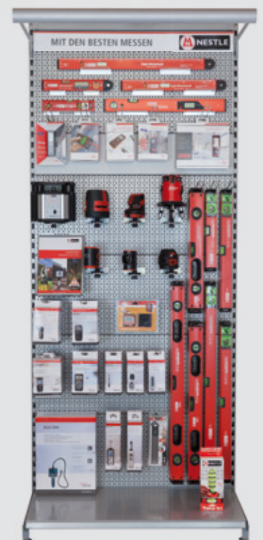
version 1m
